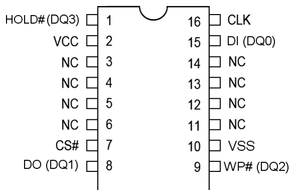
16 - LEAD SOP
