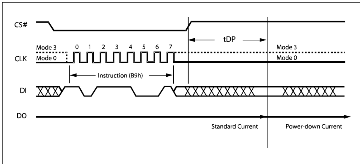
Figure 26. Deep Power-down Instruction Sequence Diagram
