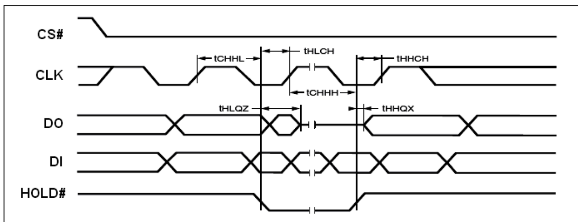
Figure 38. Hold Timing
