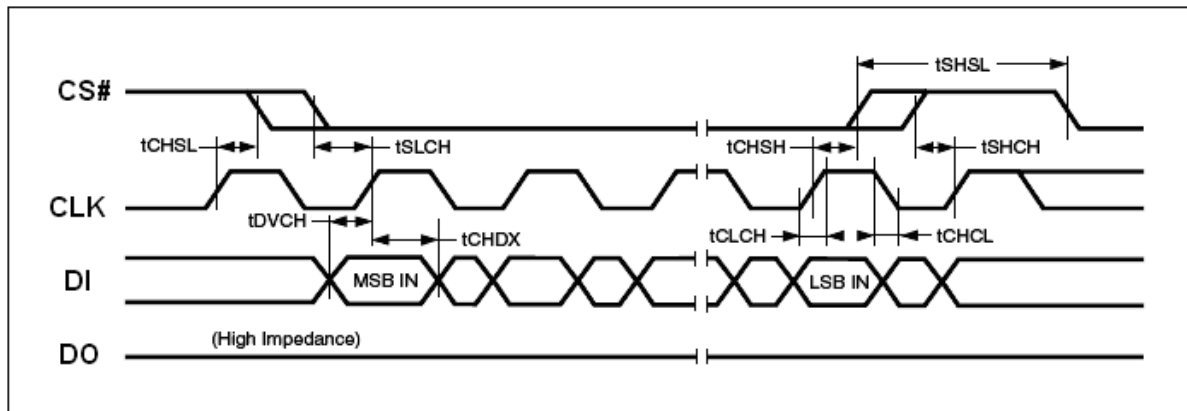
Figure 37. Input Timing
