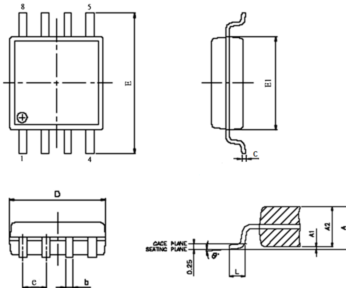
Figure 41. 8-pin SOP 200 mil (official name = 208 mil)
