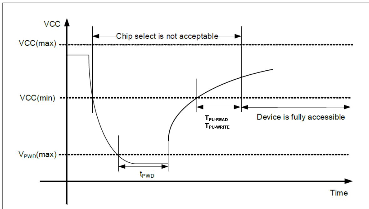
Figure 34. Power-down Timing
